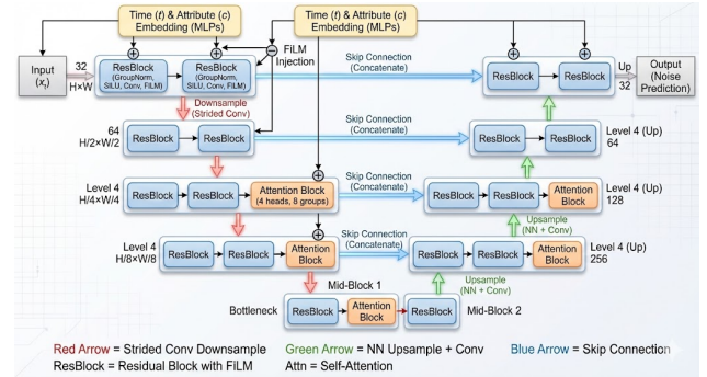
Figure 2. Architectural Overview of the Conditional U-Net.
