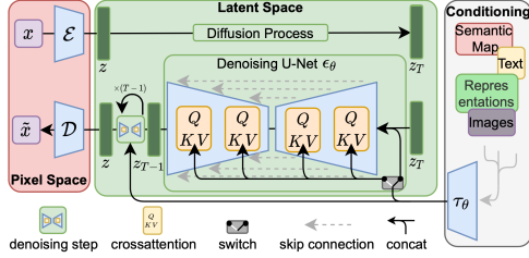
Figure 1. The architecture of the latent diffusion model (LDM). (Source: High-Resolution Image Synthesis with Latent Diffusion Models (Rombach et al., 2021))
